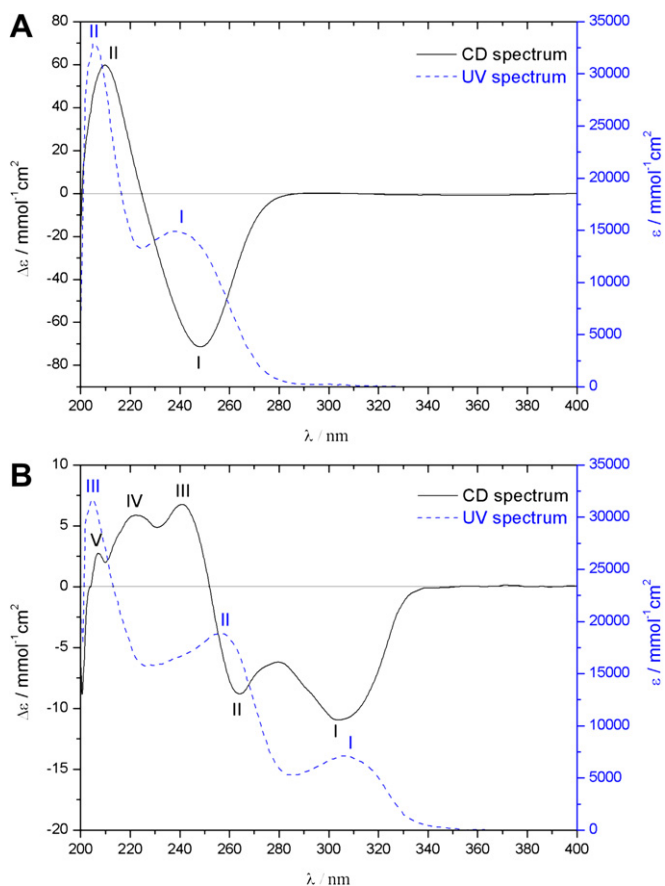
Fig. 2. A. CD (—, c = 3000 \times 10^{-5} \text{ mol dm}^{-3} , l = 1 \text{ cm} ) and UV (---, c = 2442 \times 10^{-3} \text{ mol dm}^{-3} , l = 1 \text{ cm} ) spectra of 8 in EtOH. B. CD (—, c = 2993 \times 10^{-5} \text{ mol dm}^{-3} , l = 1 \text{ cm} ) and UV (---, c = 2993 \times 10^{-5} \text{ mol dm}^{-3} , l = 1 \text{ cm} ) spectra of 7 in EtOH.
