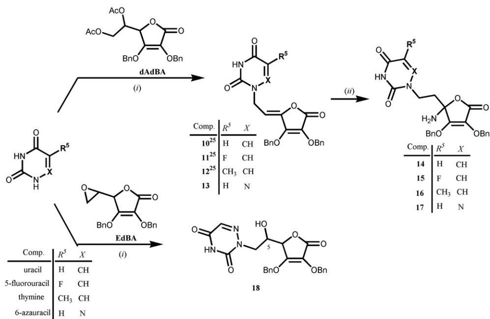
Scheme 2. Synthesis of pyrimidine derivatives of L-ascorbic acid ( 10–18 ). Reagents and conditions: (i) HMDS, (NH 4 ) 2 SO 4 /argon/reflux/3 h; TMSOTf/CH 3 CN/55–70 °C/12 h; (ii) NH 3 /MeOH-dioxane/r.t./16 h.
