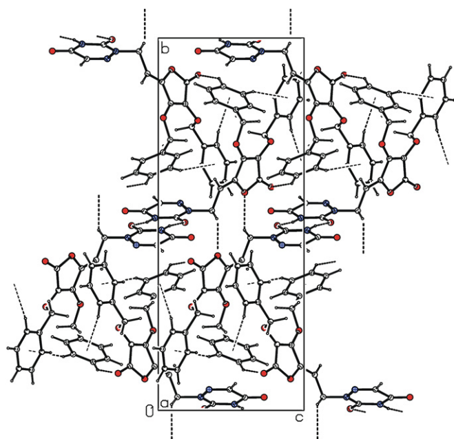
Fig. 5. A crystal packing diagram of 13 , viewed along the a axis, showing three-dimensional framework formed by one N–H...O and two C–H...O hydrogen bonds, as well as two C–H... \pi interactions. Hydrogen bonds and C–H... \pi interactions are indicated by dashed lines.
