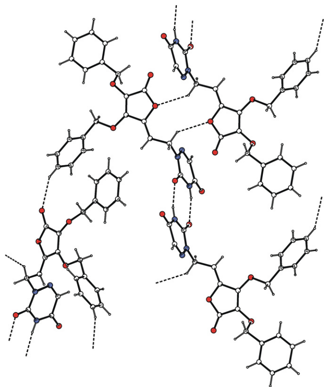
Fig. 4. A part of the crystal structure of 13 , showing N–H...O and C–H...O hydrogen bonds. Hydrogen bonds are indicated by dashed lines.
