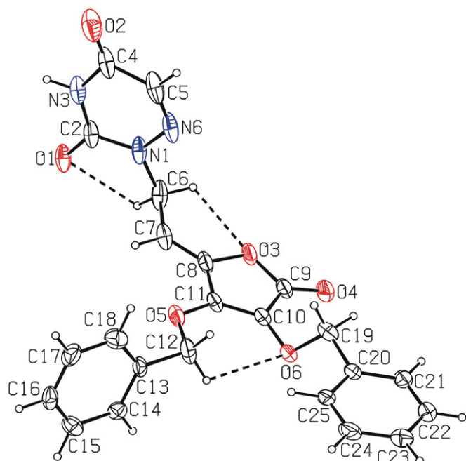
Fig. 3. A view of 13 , with the atom-numbering scheme. Displacement ellipsoids for non-hydrogen atoms are drawn at the 20% probability level. Intramolecular hydrogen bonds are indicated by dashed lines.
