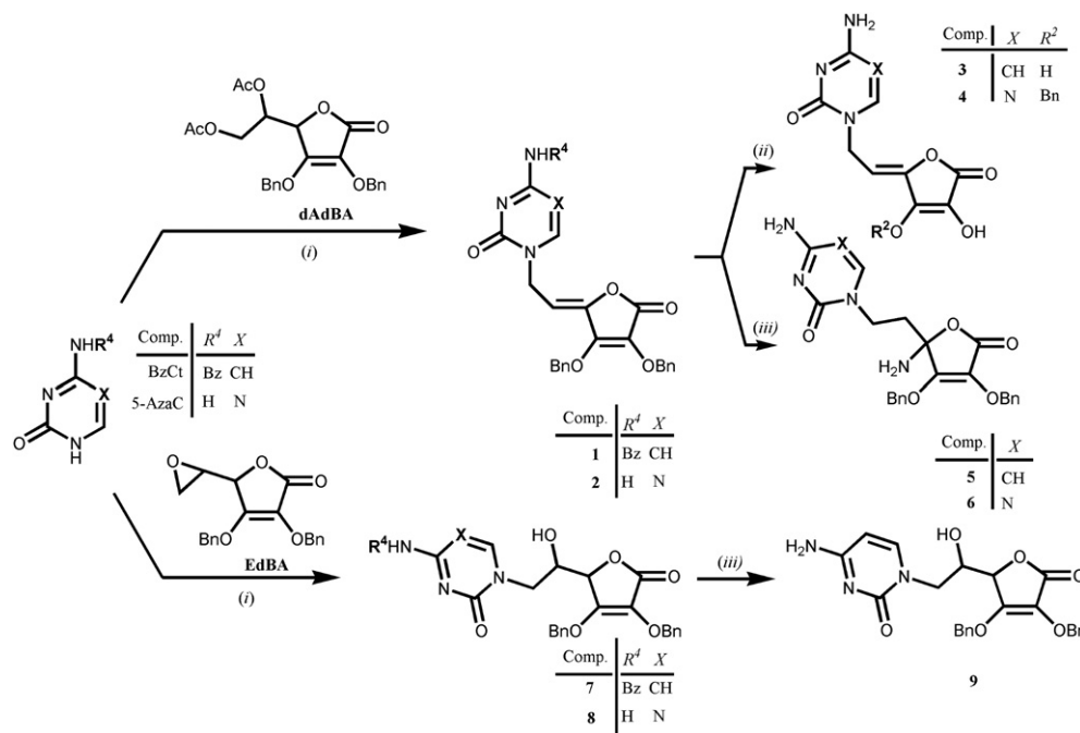
Scheme 1. Synthesis of cytosine and 5-azacytosine derivatives of L -ascorbic acid ( 1–9 ). Reagents and conditions: (i) HMDS, (\text{NH}_4)_2\text{SO}_4 /argon/reflux/3 h; TMSOTf/ \text{CH}_3\text{CN}/55-70^\circ\text{C}/12 h; (ii) \text{BCl}_3/\text{CH}_2\text{Cl}_2/-78^\circ\text{C}/2 h; (iii) \text{NH}_3/\text{MeOH} -dioxane/r.t./16 h.
