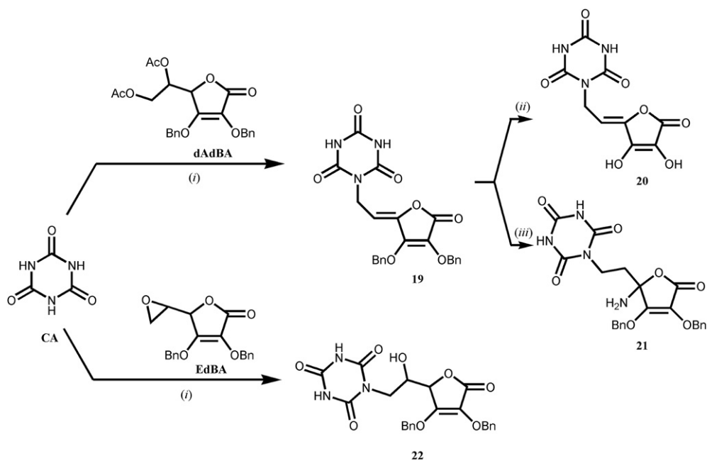
Scheme 3. Synthesis of cyanuric acid derivatives of L-ascorbic acid ( 19–22 ). Reagents and conditions: (i) HMDS, (NH 4 ) 2 SO 4 /argon/reflux/3 h; TMSOTf/CH 3 CN/55–70 °C/12 h; (ii) BCl 3 /CH 2 Cl 2 /–78 °C/2 h; (iii) NH 3 /MeOH-dioxane/r.t./16 h.
